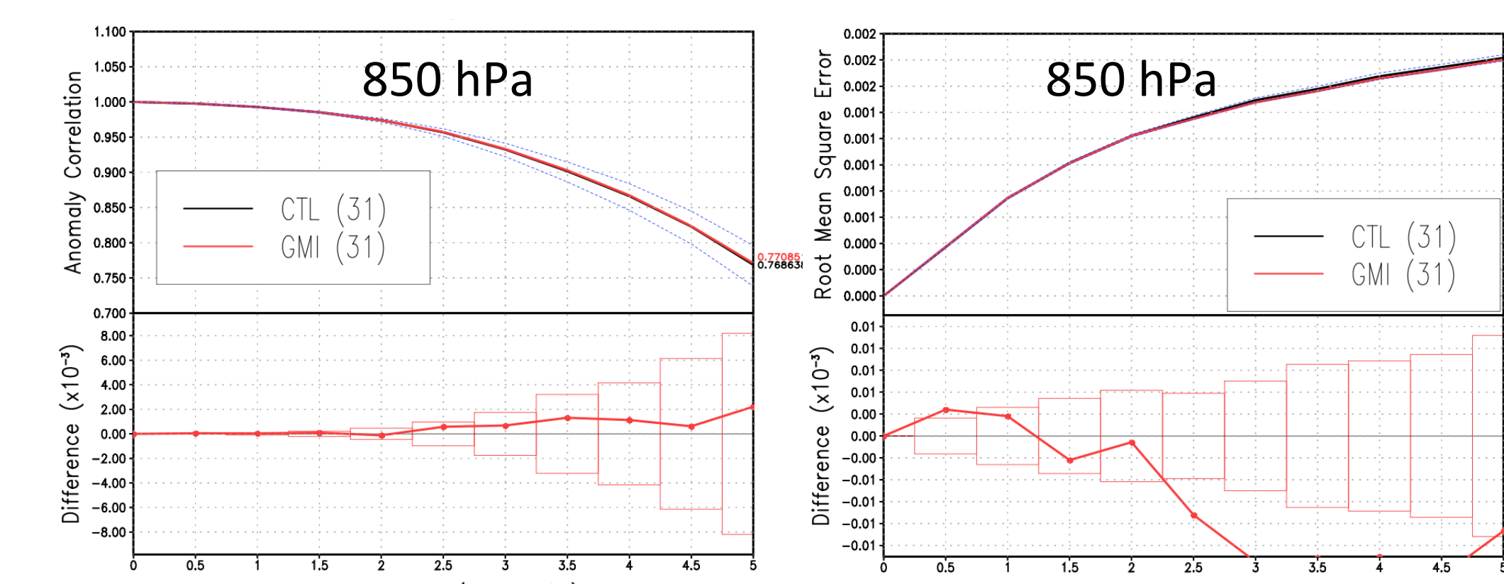
Fig 7. (Left) Forecast scores of global correlations of geo-potential height anomalies in forecasts and in GEOS-5 analysis at 850 hPa. The forecasts are performed using GEOS-5 analyses with (GMI experiment) and without (control) GMI data. (Right) Forecast scores of root mean square error in moisture distributions at 850 hPa. The forecast scores' improvement is neutral in geo-potential heights, and is slightly significant in moisture field after 3 days.
