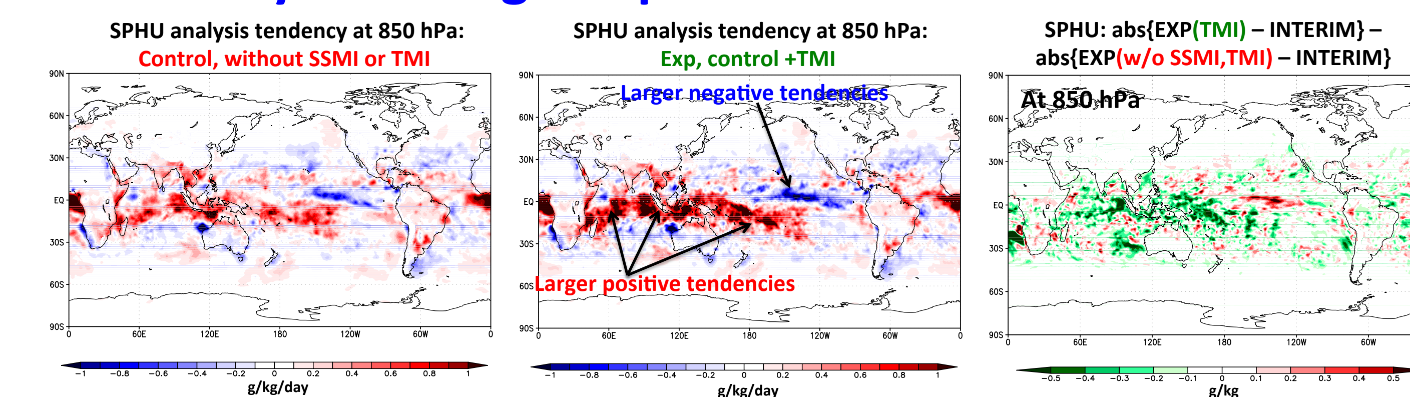
Fig 9. Specific humidity tendencies in (left) control experiment and (middle) TMI experiment at 850 hPa in January 2005. Right panel shows a comparison of the absolute specific humidity differences between GEOS-5 analyses and ECMWF Interim data set. Red and green colors suggest control and TMI experiments are close to Interim data set, respectively. The right panel demonstrates TMI observations make GEOS-5 specific analysis closer to ECMWF Interim data set.
